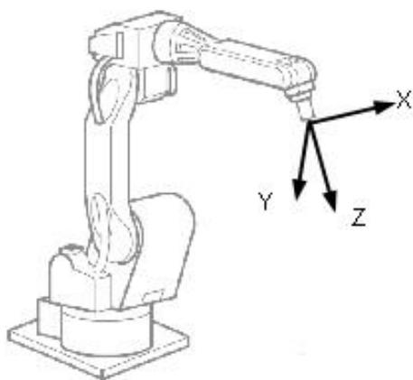
Figure 1: Tool Coordinate System
